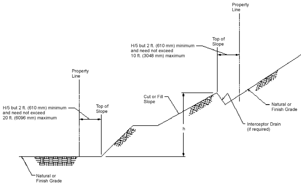
FIGURE J108.1 DRAINAGE DIMENSIONS
