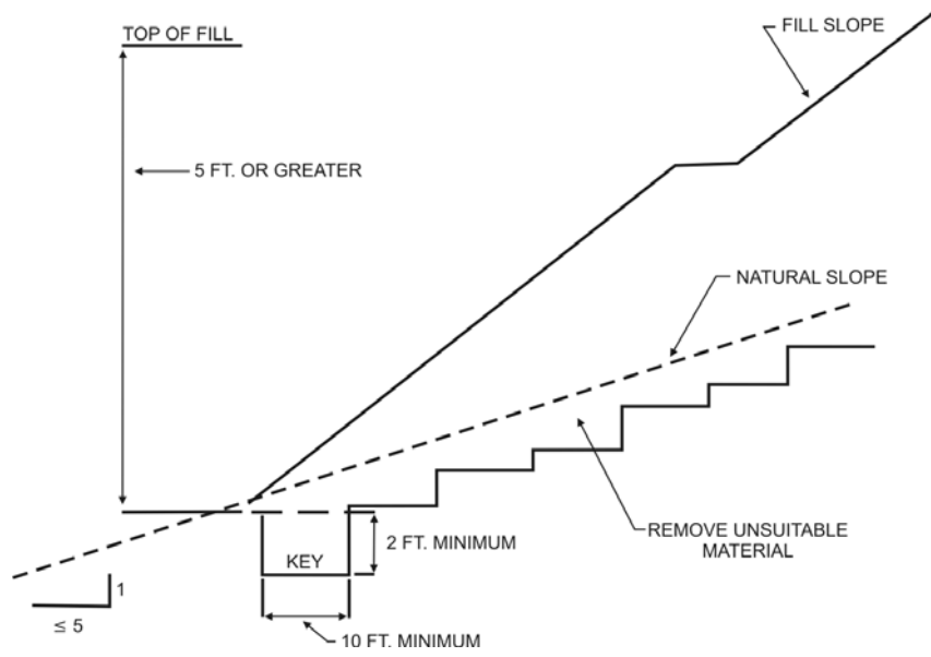
FIGURE J107.3 BENCHING DETAILS
